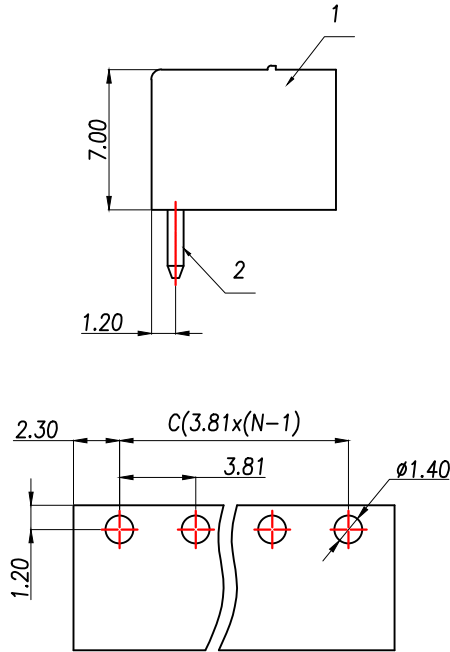
PCB LAYOUT
