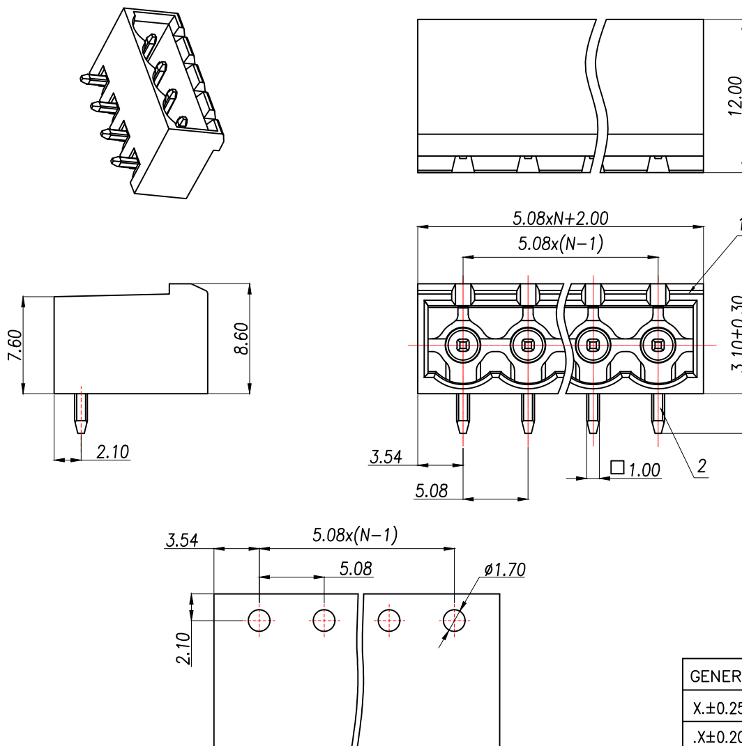
PCB LAYOUT
