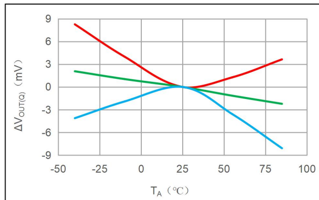
ΔVOUT(Q) vs TA [1]
