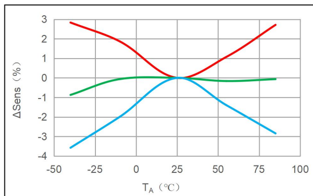
Δ Sens vs TA [1]
