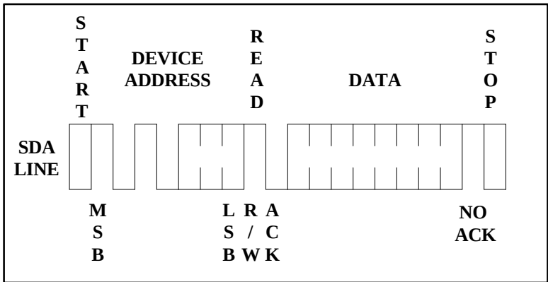
Figure 9. Random Read
