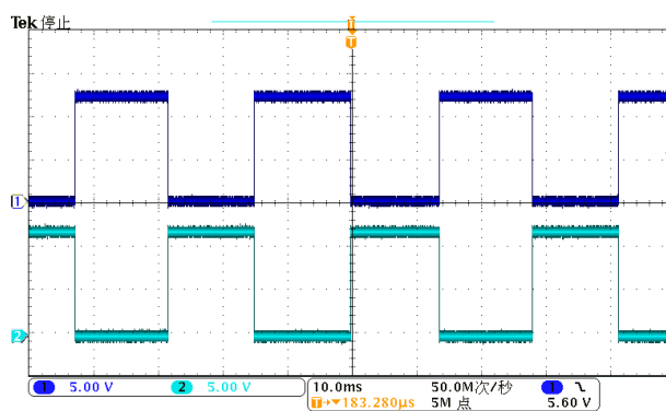
DO/DOB @ V_{DD}=12V
