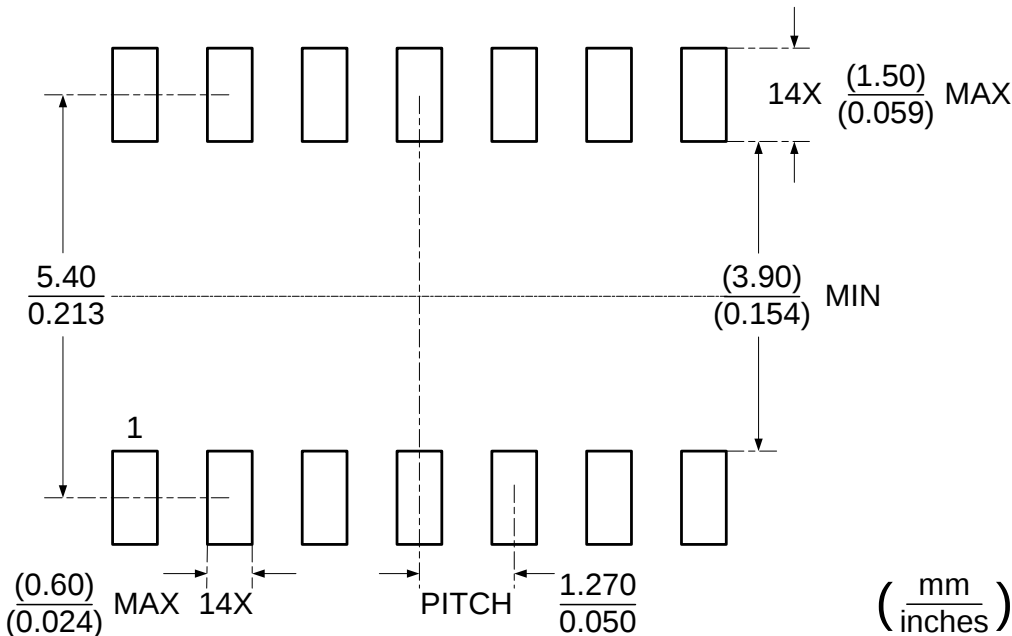
RECOMMENDED SOLDERING FOOTPRINT, SOIC-14L
