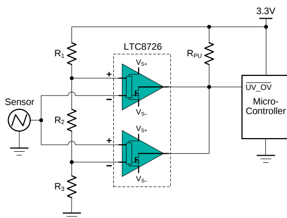
Figure 6. Window Comparator
