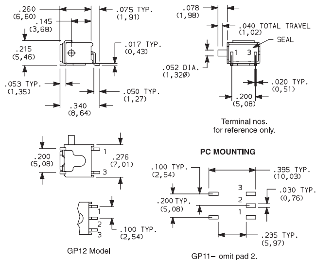
GP11MSABE SPST
