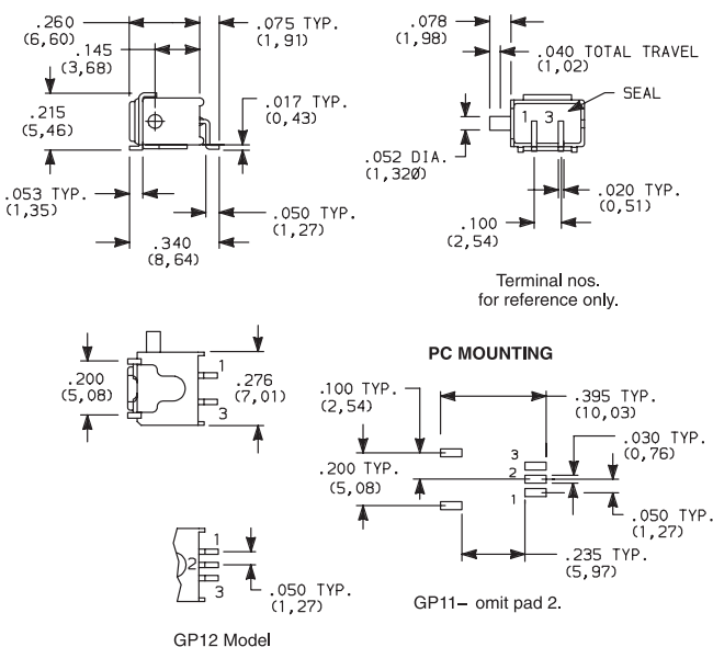
GP11MSA1BE SPST
