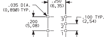
PC MOUNTING
