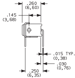
PC MOUNTING
