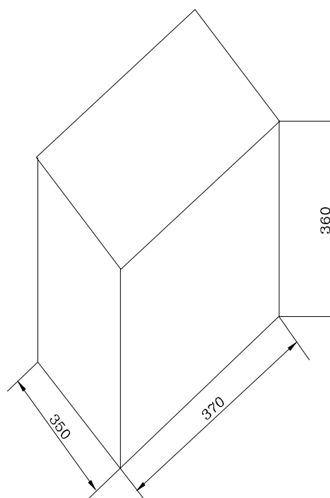
CARTON BOX 10 INNER BOX 5K PCS BUZZER
