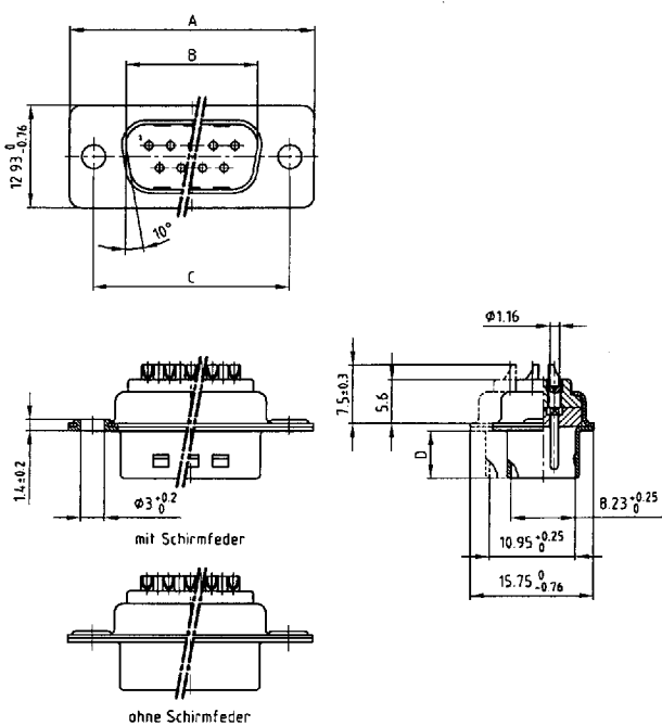
Plug connector
