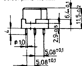
Solder pin Ø 1.0 mm
