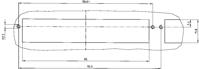
Panel cutout
