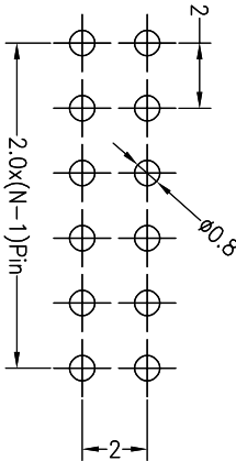
Recommended P.C.B Layout(Top Side) (PCB BOARD TOLERANCE±0.05)
