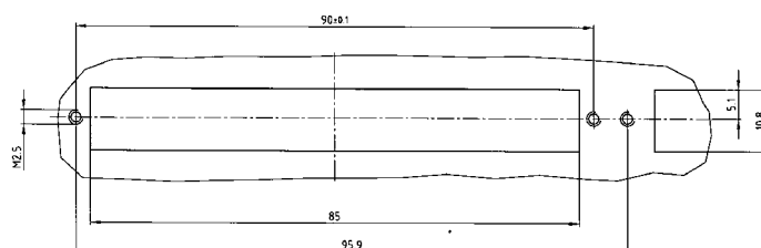
Panel cutout
