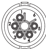
5 POSITION B-KEY #26 PIN & SOCKET CONTACT
