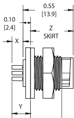
17X80-XXG-3XX PANEL MOUNT CONNECTOR CRIMP
