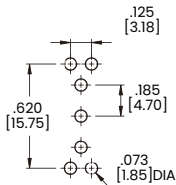
P.C.MOUNTING
