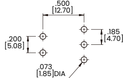
P.C.MOUNTING
