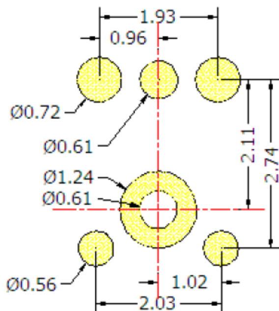
Recommended Solder Pad Layout
