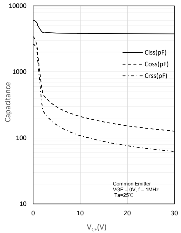
Fig. 10 Capacitance characteristics
