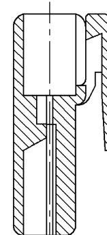
SEC. B-B
