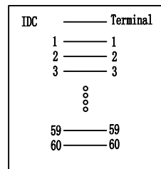
Pin assignment
