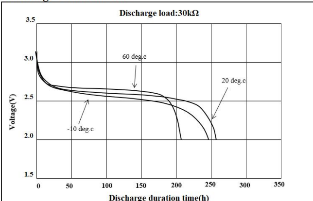
Discharge Characteristics
