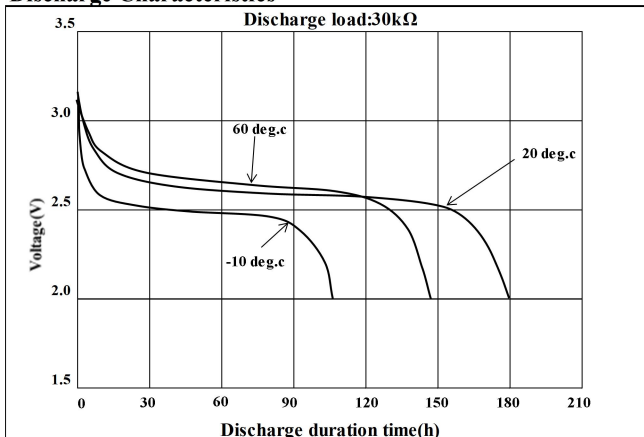
Discharge Characteristics
