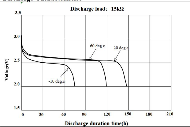
Discharge Characteristics
