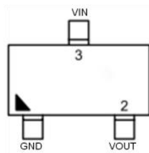
Pin Configurations
