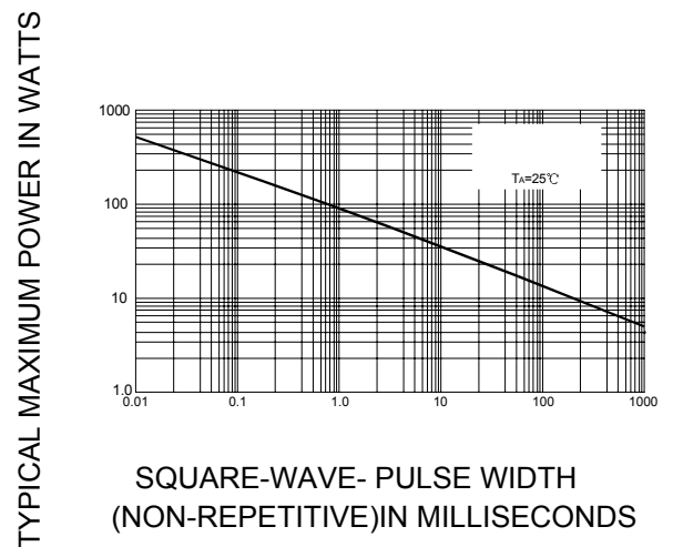
FIG.2 – TRANSIENT SURGE CAPABILITY
