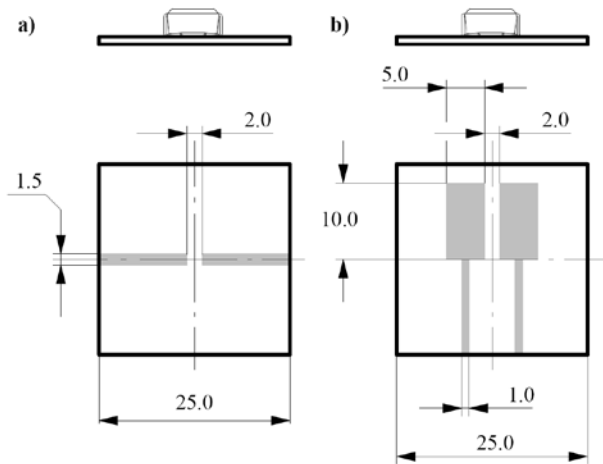
Figure 1. Boards for R_{thJA} definition (conner overlav 35μ)
