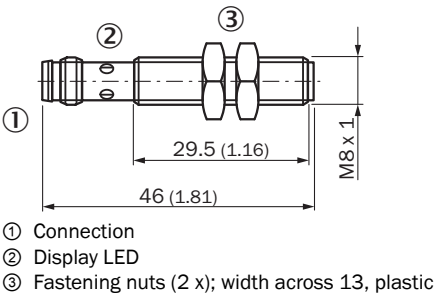
MM08, connector, short-body housing
