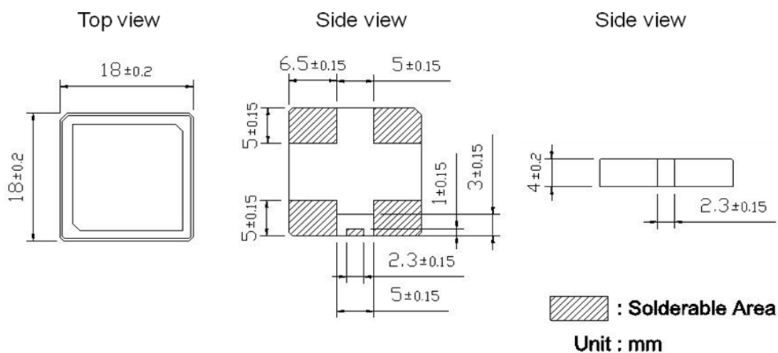
Fig. 1 Mechanical Data
