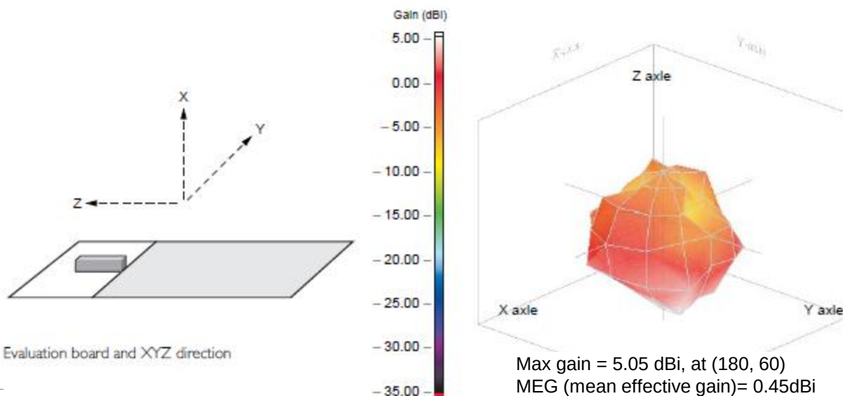
Radiation pattern
