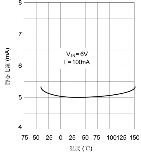
Ground端电流
