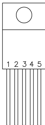
TO220T-5
