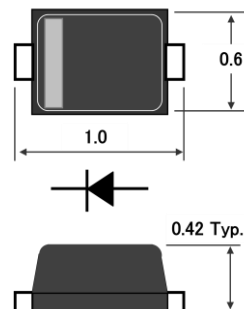
SOD-923 Unit: mm
