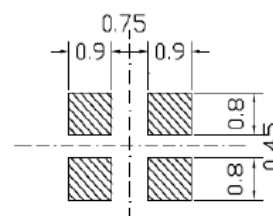
LAND PATTERN (REFERENCE)
