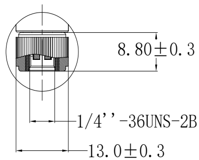
SMA-Female DETAIL A
