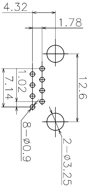
PCB LAYOUT
