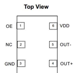
Figure 1. Pin Assignments
