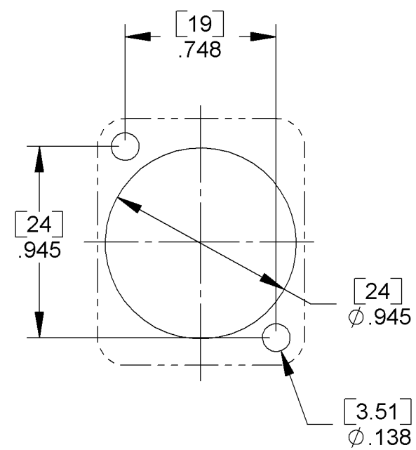
PANEL CUT-OUT FRONT OR REAR MOUNT
