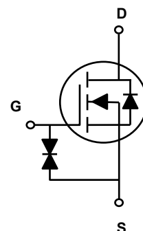
Schematic Diagram
