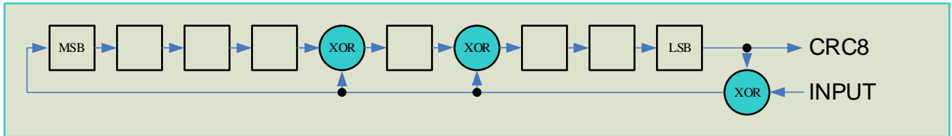
Figure 9. CRC Generator
