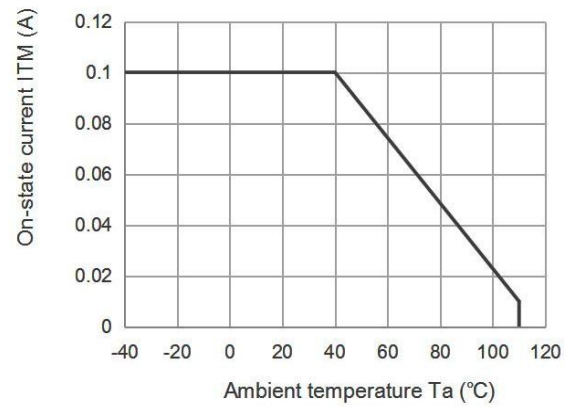
Fig.2 On-state current vs. Ambient temperature
