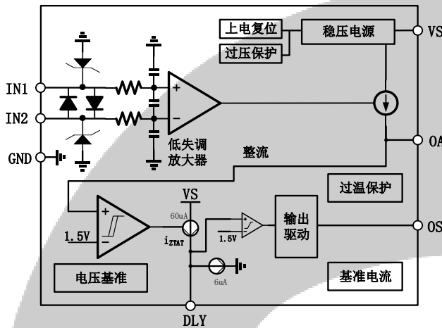
Figure 5. SS54123H Block Diagram
