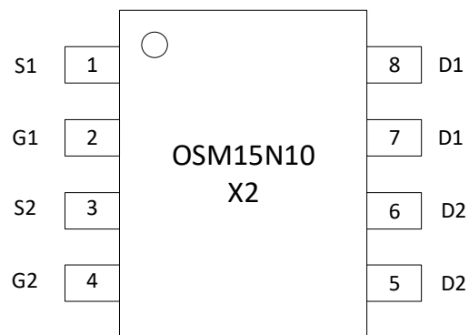
Figure 2. Pin Configuration (Bottom View)
