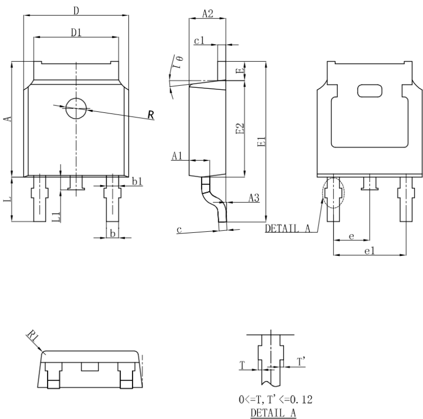
Figure 4. Package Level Package [PLP]
