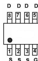
pin assignment
