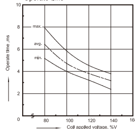
Operate time
