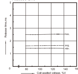
Release time
