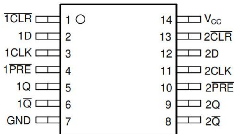
Figure 2.1: Top View
