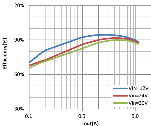
Efficiency & I out (%)
