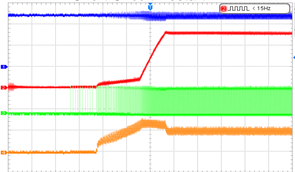
Short Circuit Restart
