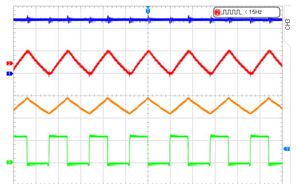
5A Load Test
