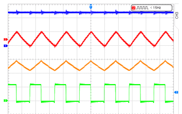
3A Load Test
