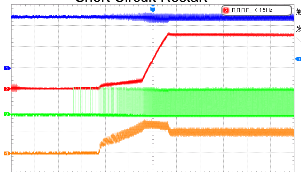
Short Circuit Restart
