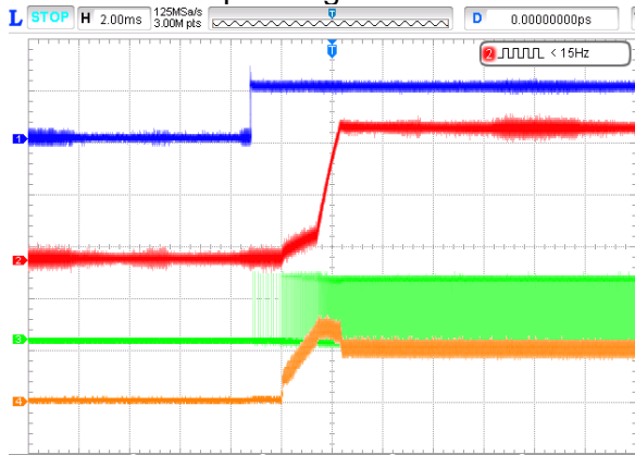
Startup through Enable
