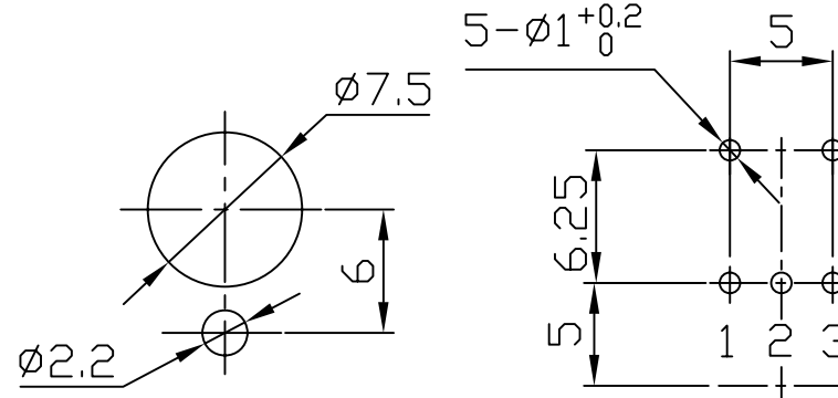
Mounting hole detail
