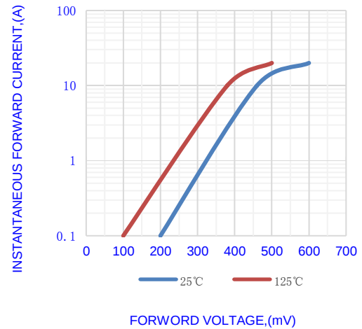
Fig.2-TYPICAL INSTANTANEOUS FORWARD
