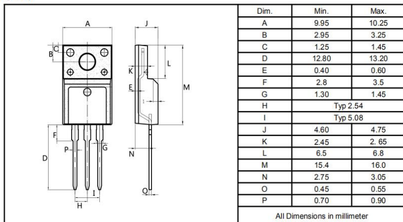
TO-220F
