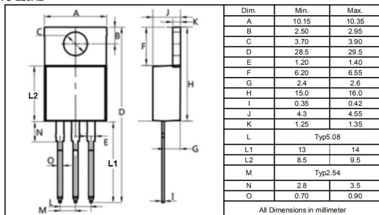
TO-220AB
