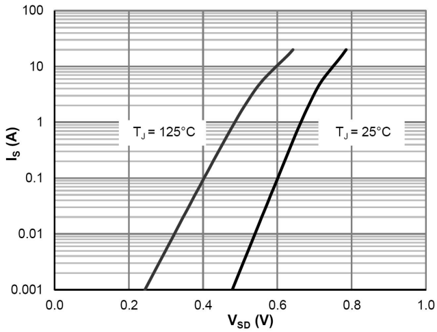
Body-Diode Characteristics
