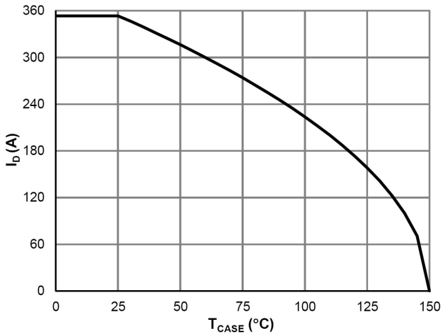
Current De-rating
