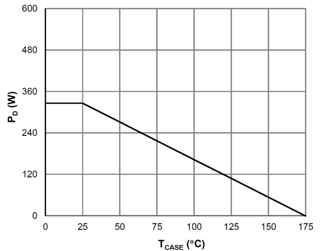
Power De-rating
