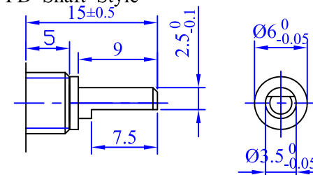
FD Shaft Style
