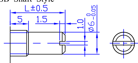
SB Shaft Style
