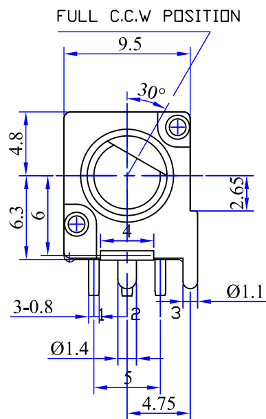
FB Shaft Style
