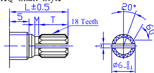
KQ Shaft Style
